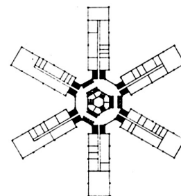
TYPICAL PLAN OF OFFICE TOWERS. ACCOMMODATION FOR 18,000 PERSONS APPROXIMATELY. ALL VERTICAL SERVICES ARE CARRIED IN THE CENTRAL TOWERS.
