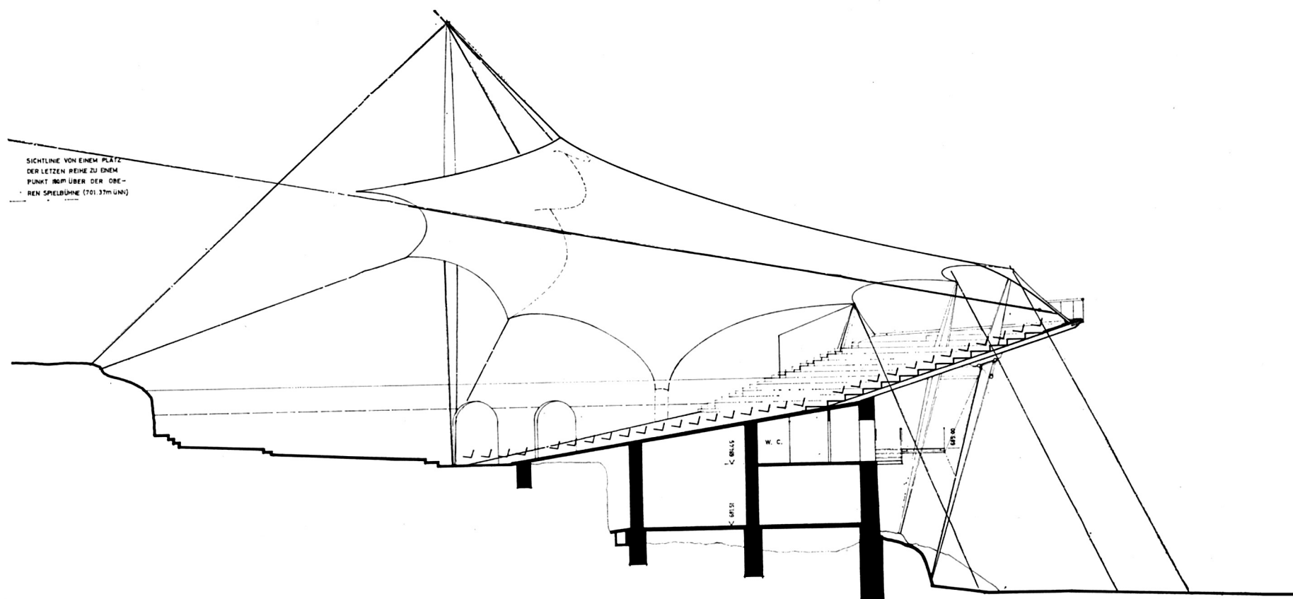
Section, showing extension of the stands
